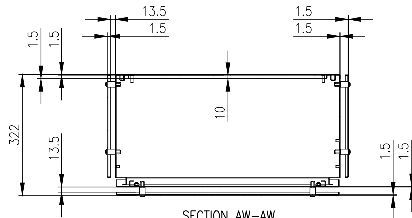
SECTION AW-AW
